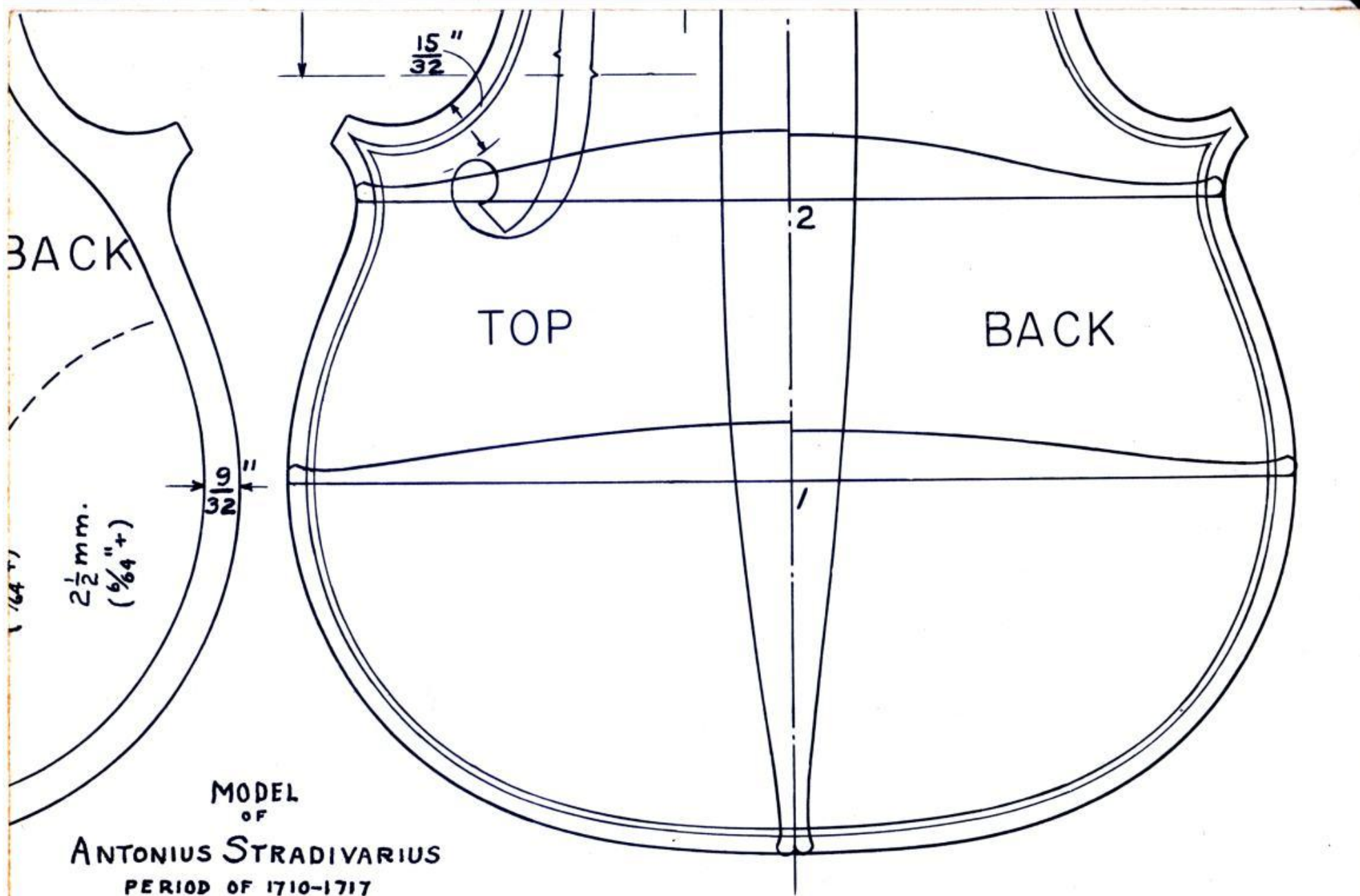
ARCHING GUIDES
